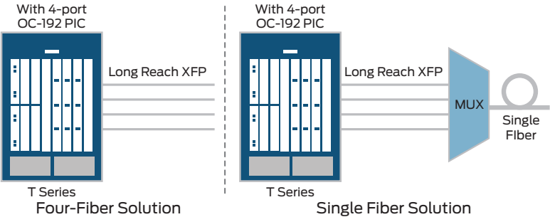
By using inverse multiplexing, four OC-192 ports can be aggregated to a full OC-768 frame
